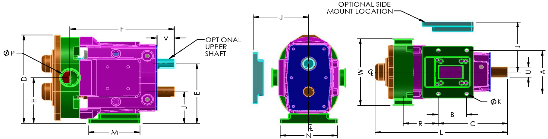
ZMT ZDE U2 Evolution Dimensions and Weights
