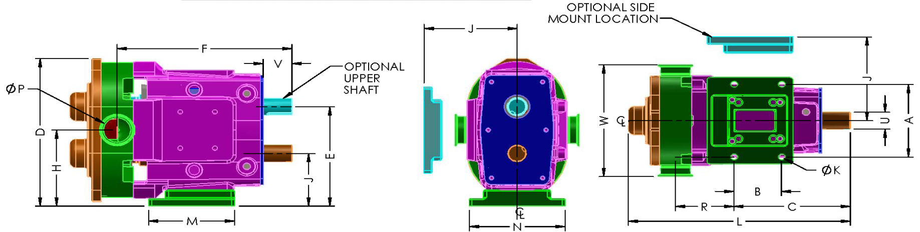
ZMT ZDU1 Dimensions and Weights
